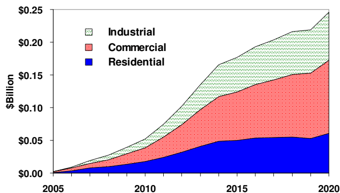
Cumulative Energy Bill Savings in New Mexico*
