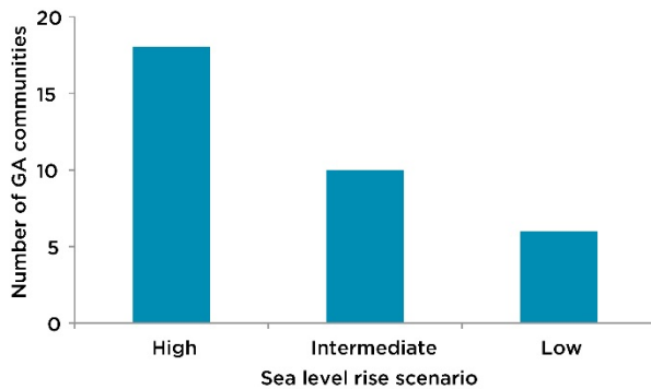
FIGURE 2. Number of Chronically-Inundated Communities In Georgia In 2100 Under Three Scenarios.
